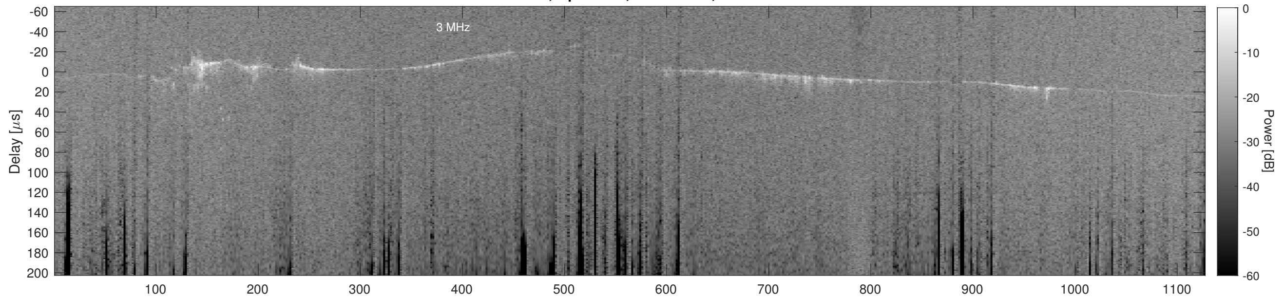
Orbit 22901, Cluttergram
