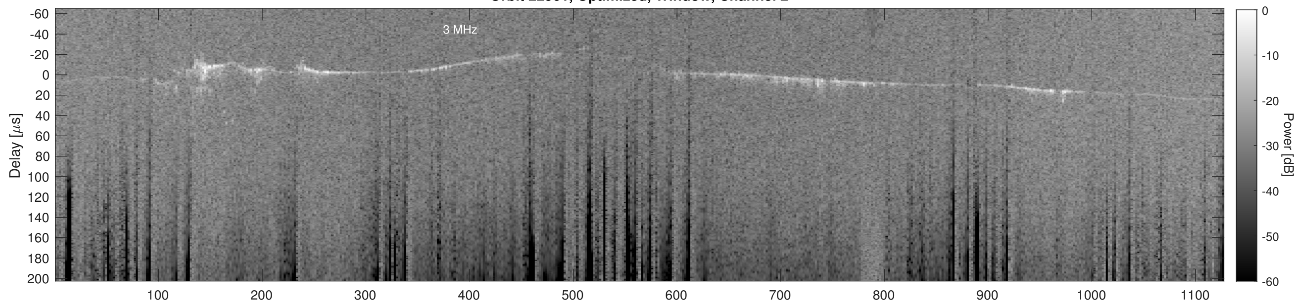
Orbit 22901, Cluttergram
