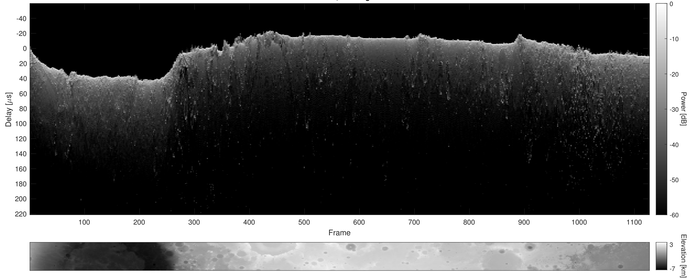
Orbit 22903, Cluttergram
