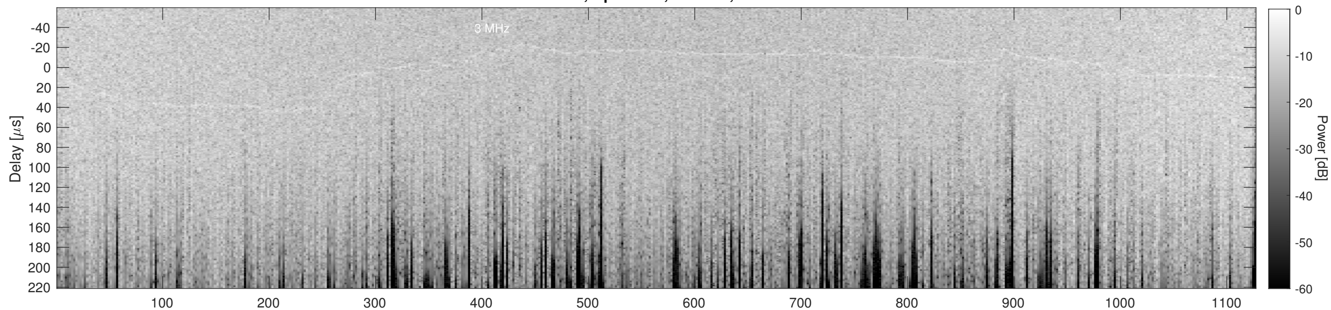
Orbit 22903, Cluttergram
