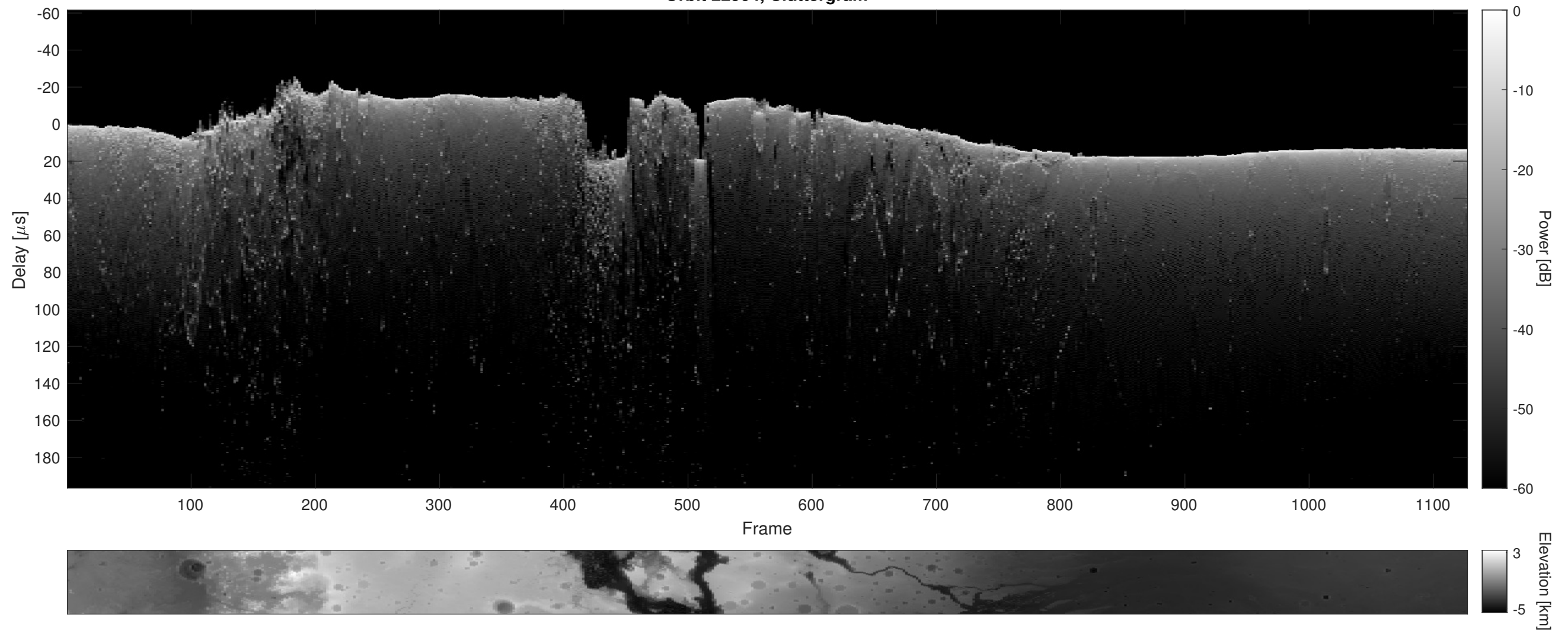
Orbit 22904, Cluttergram
