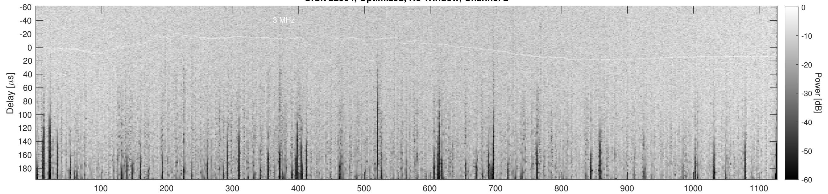
Orbit 22904, Cluttergram
