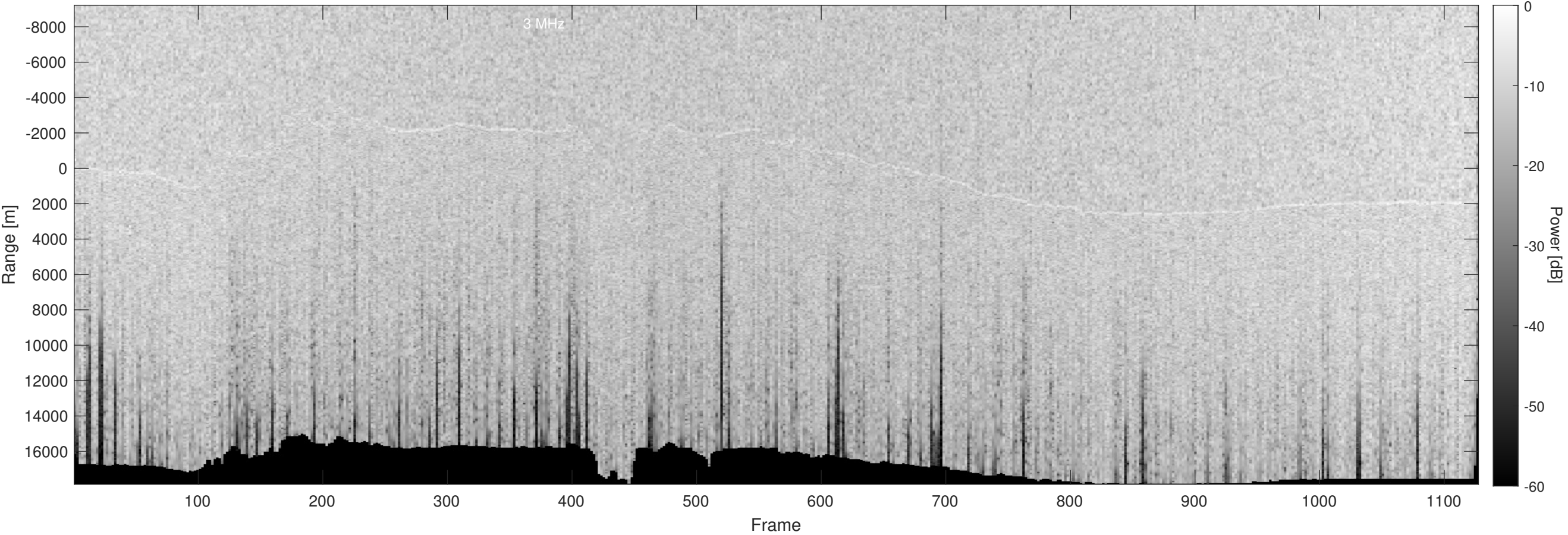
Orbit 22904, Optimized, No Window, Depth-Corrected, Channel 2
