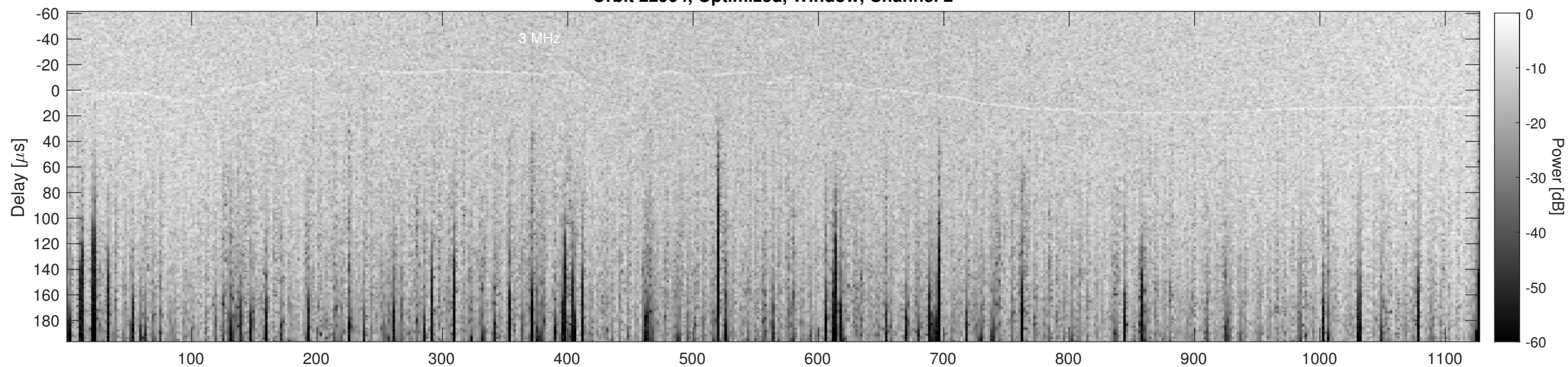
Orbit 22904, Cluttergram
