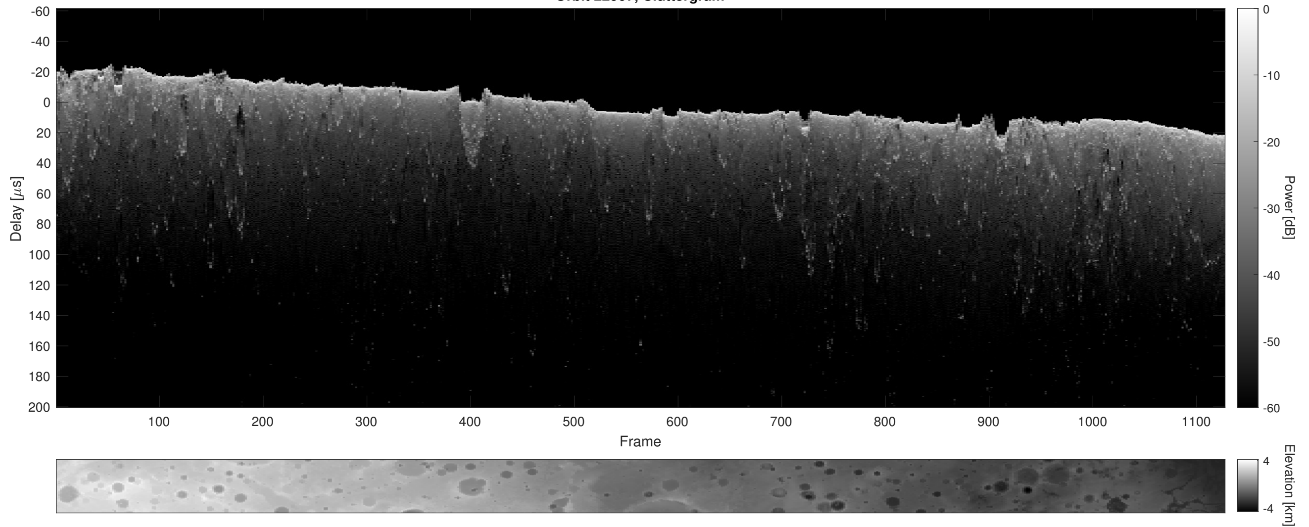
Orbit 22907, Cluttergram
