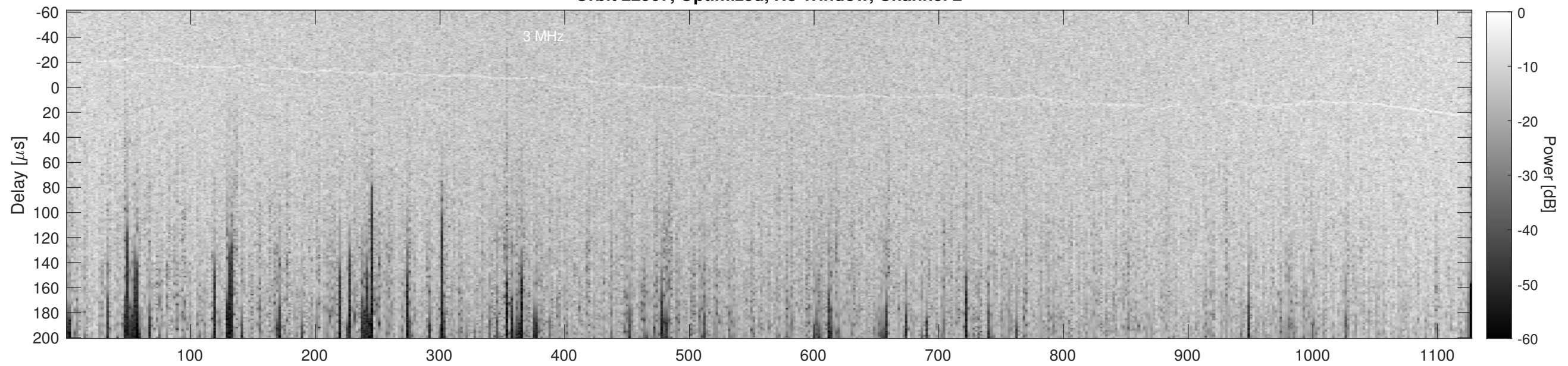
Orbit 22907, Cluttergram
