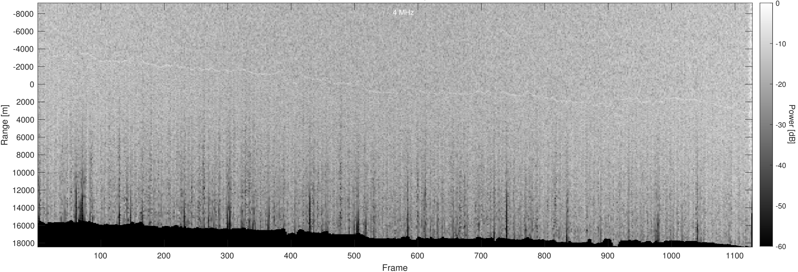
Orbit 22907, Optimized, No Window, Depth-Corrected, Channel 2
