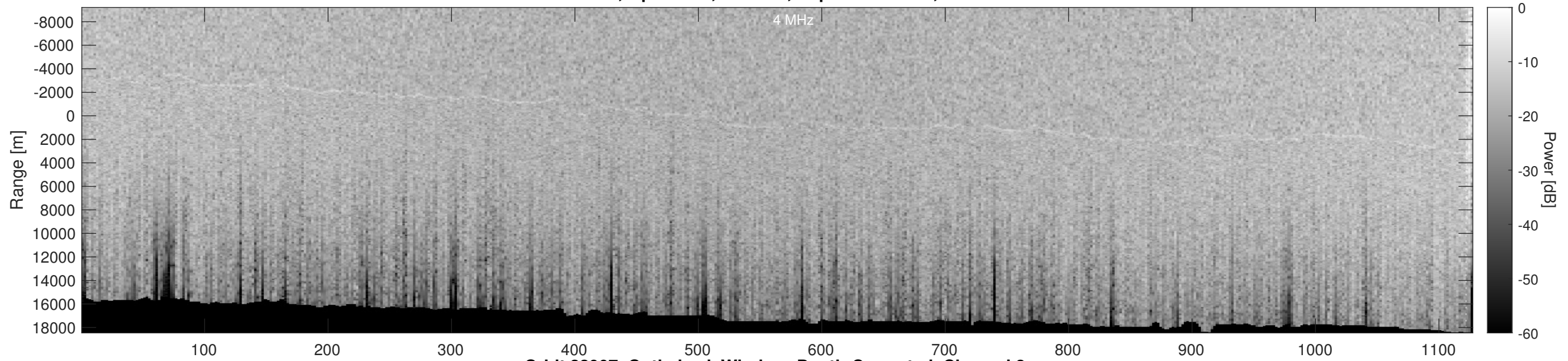
Orbit 22907, Optimized, Window, Depth-Corrected, Channel 2
