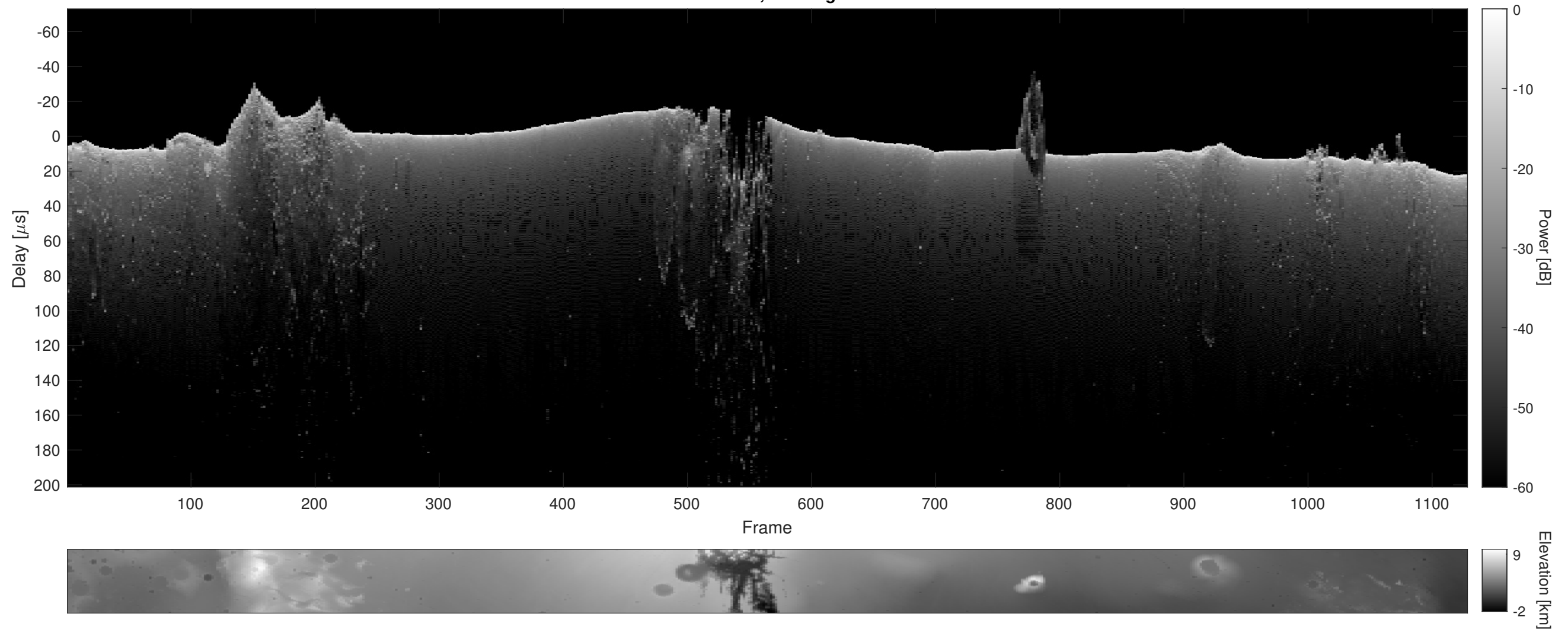
Orbit 22908, Cluttergram
