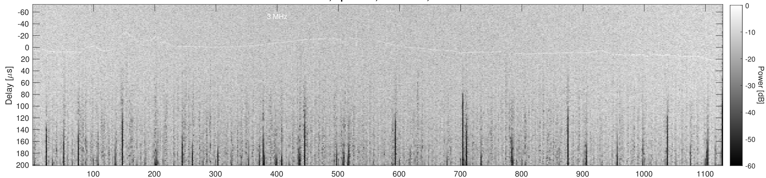
Orbit 22908, Cluttergram
