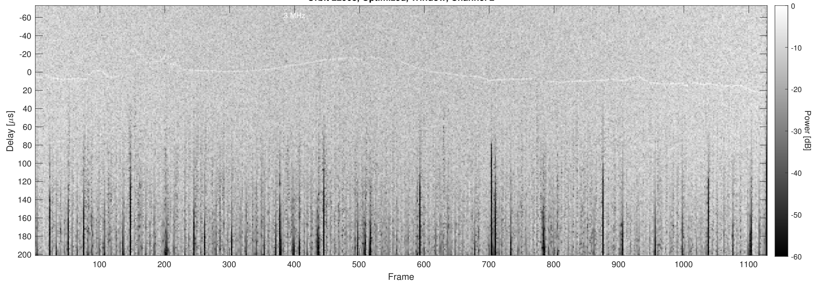
Orbit 22908, Optimized, Window, Channel 2
