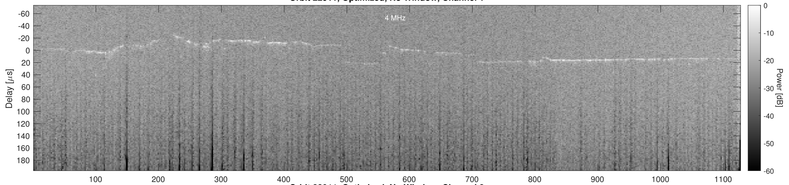
Orbit 22911, Optimized, No Window, Channel 2
