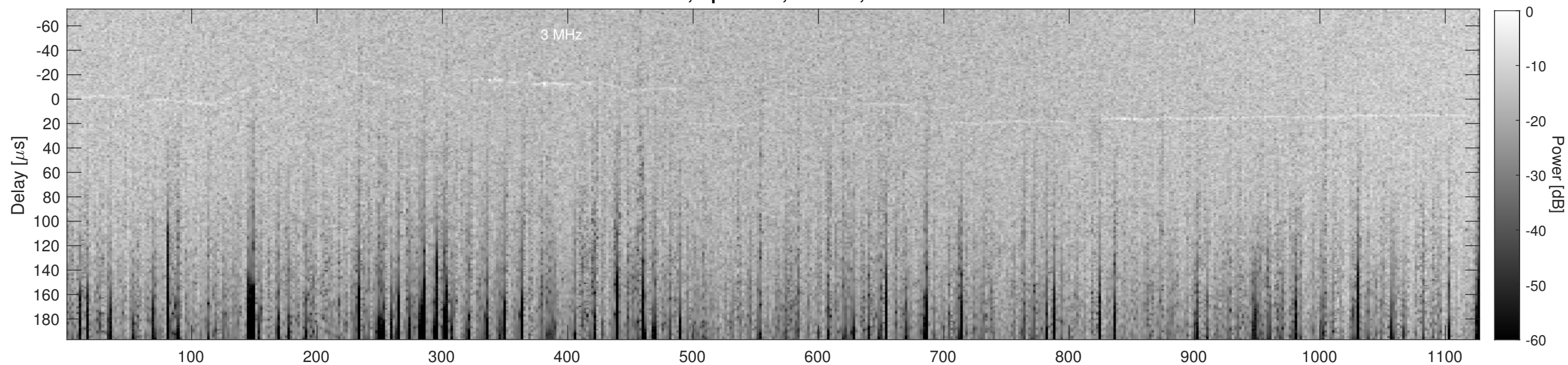
Orbit 22911, Cluttergram
