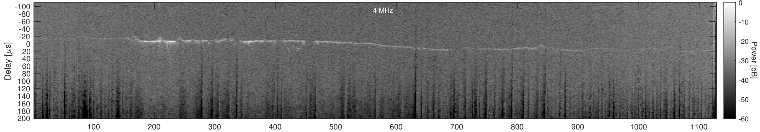
Orbit 22912, Cluttergram
