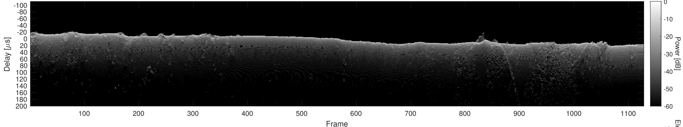
Orbit 22912, Cluttergram
