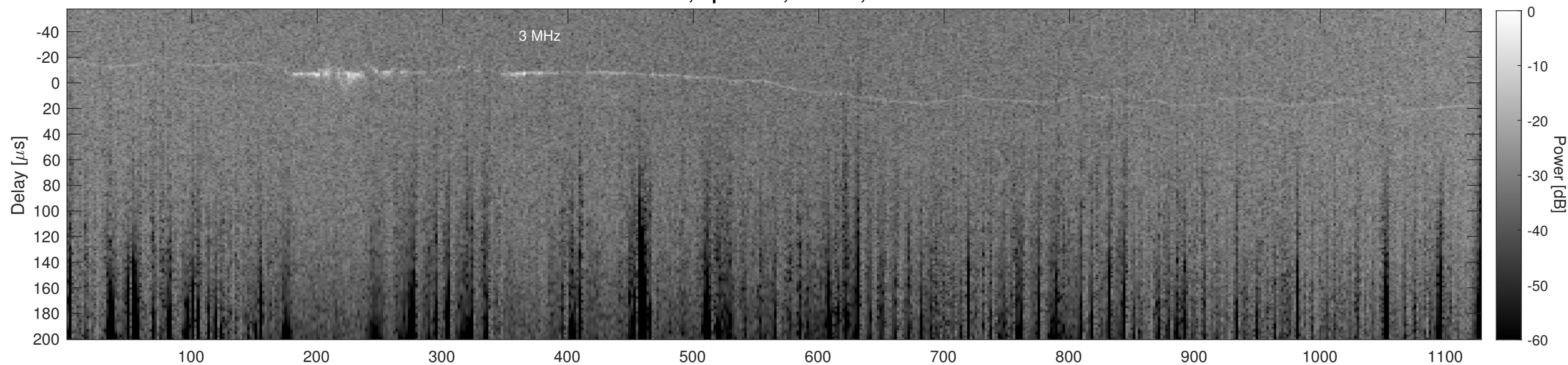
Orbit 22912, Cluttergram
