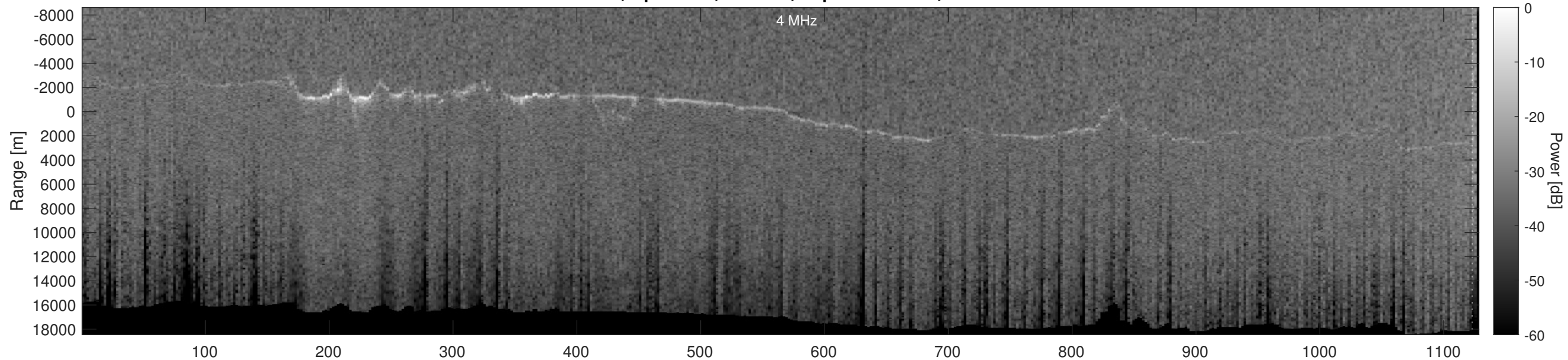
Orbit 22912, Optimized, Window, Depth-Corrected, Channel 2
