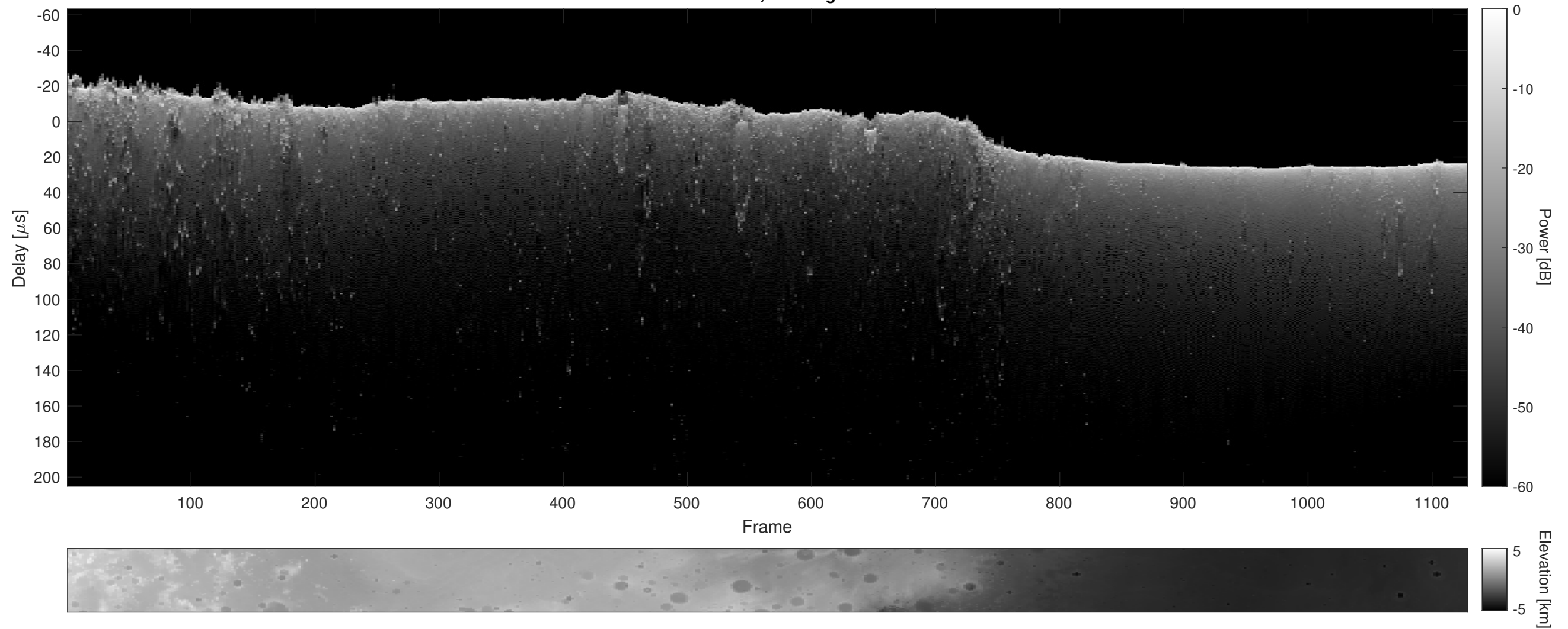
Orbit 22915, Cluttergram
