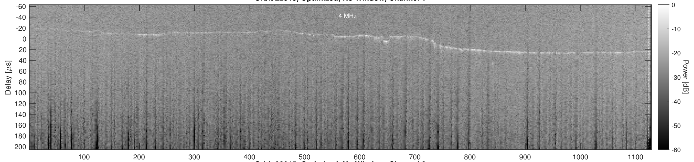
Orbit 22915, Optimized, No Window, Channel 2
