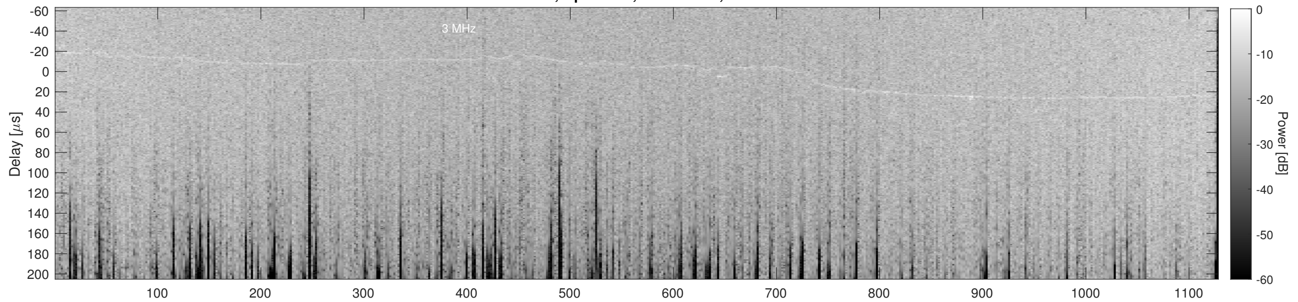
Orbit 22915, Cluttergram
