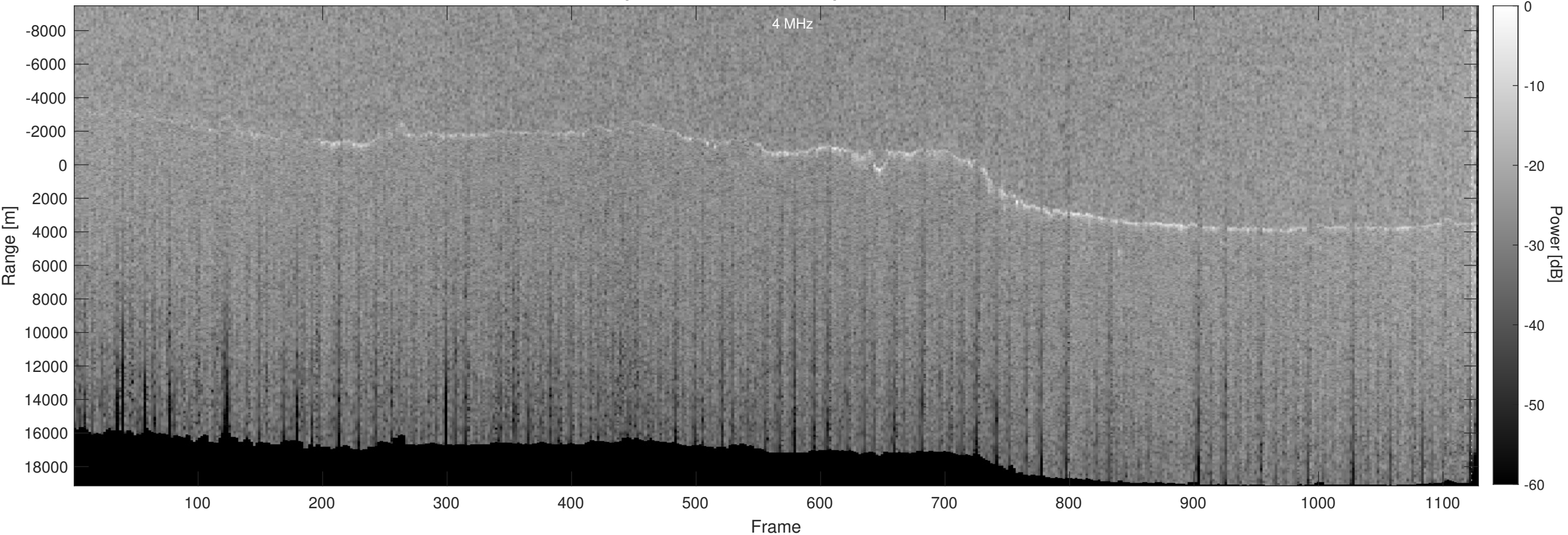
Orbit 22915, Optimized, No Window, Depth-Corrected, Channel 2
