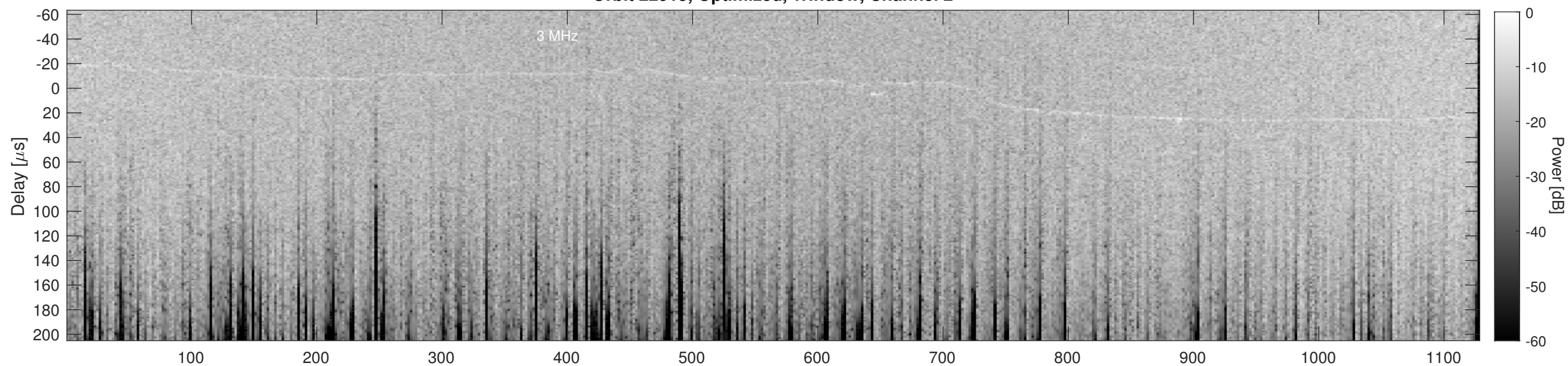
Orbit 22915, Cluttergram
