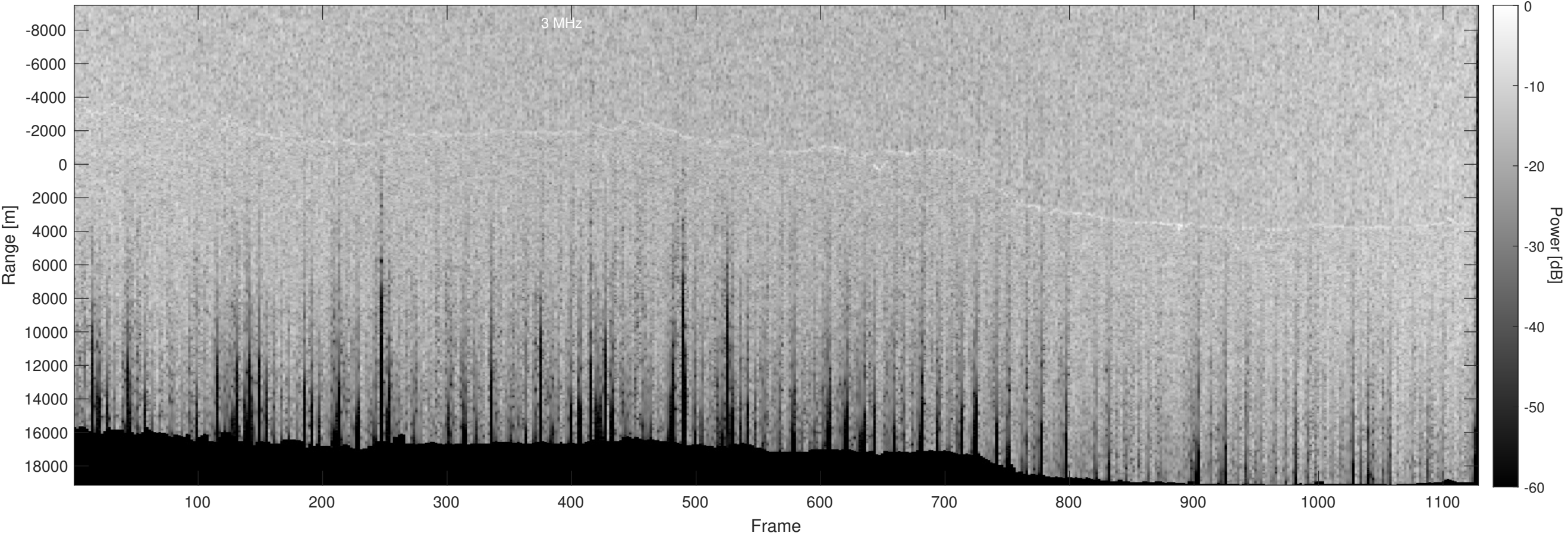
Orbit 22915, Optimized, Window, Depth-Corrected, Channel 2
