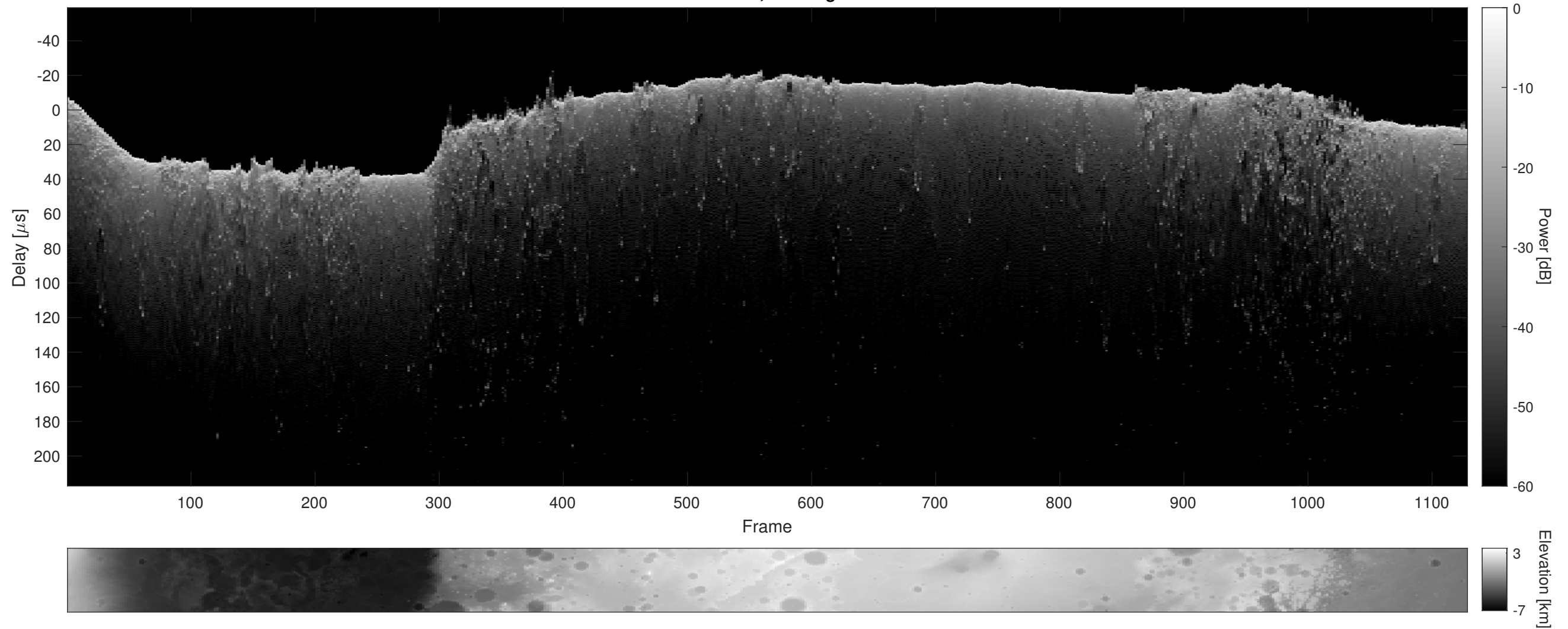
Orbit 22917, Cluttergram
