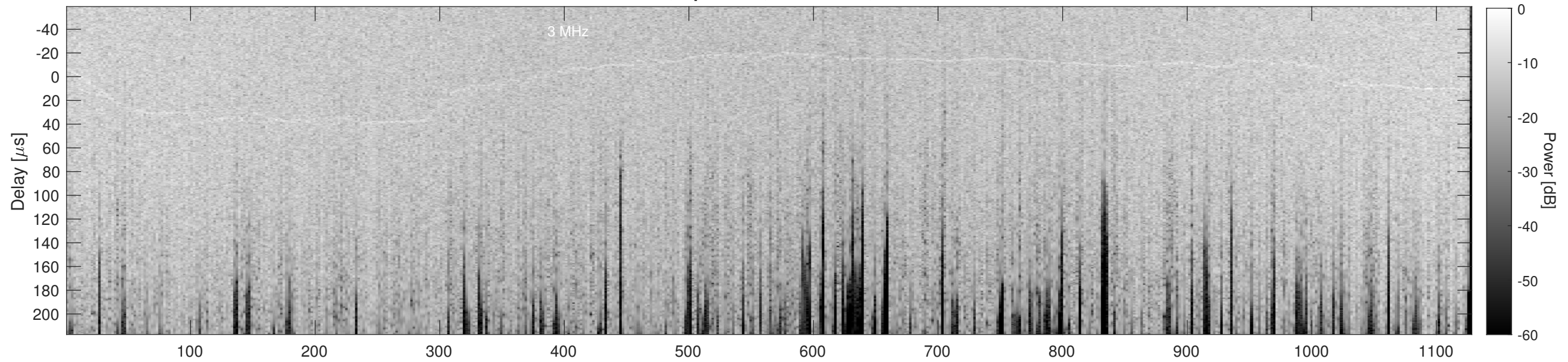
Orbit 22917, Cluttergram
