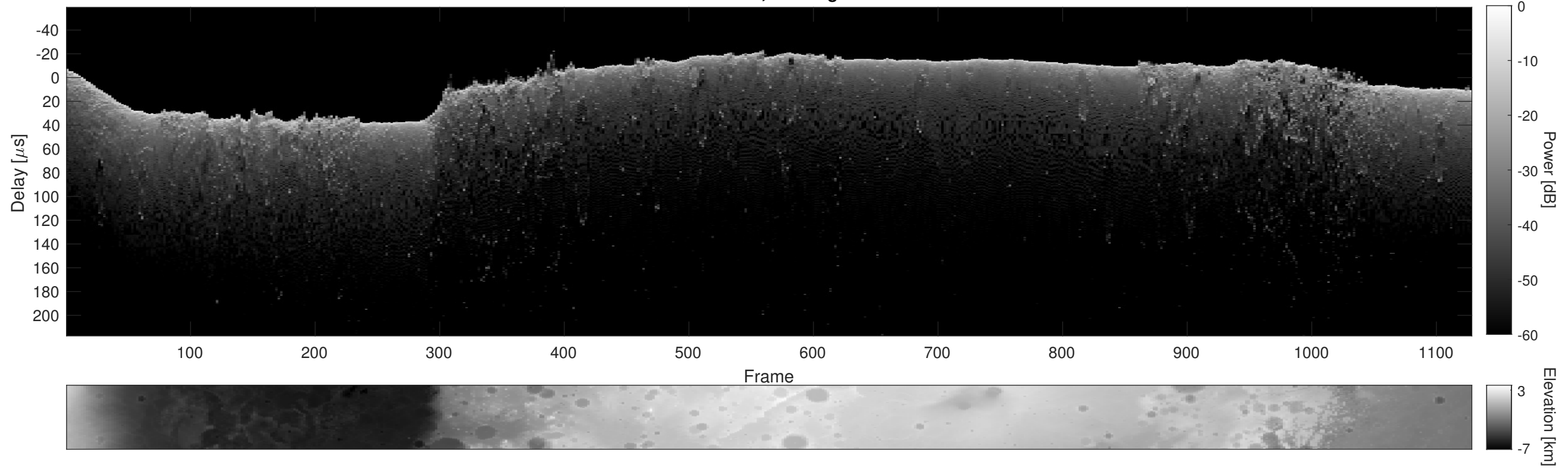
Orbit 22917, Cluttergram
