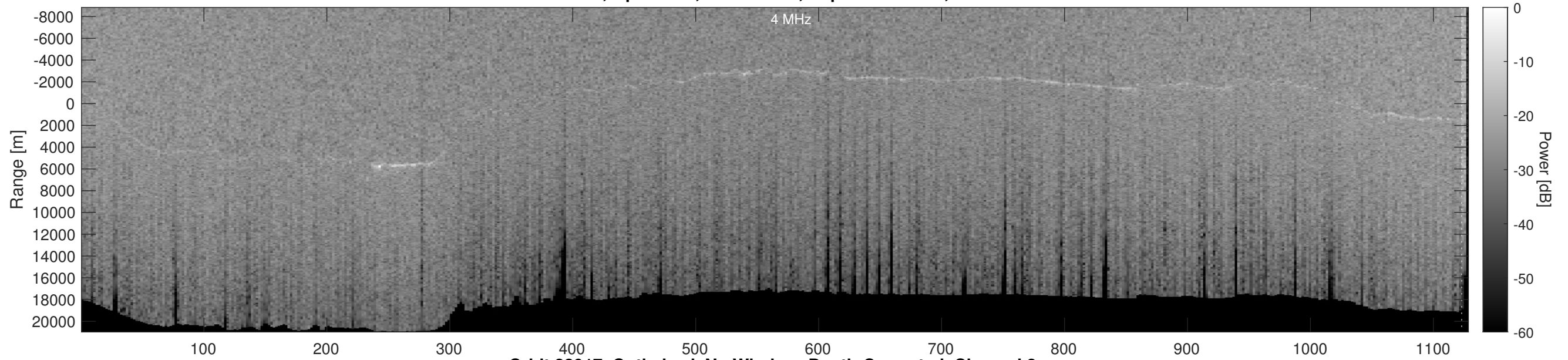
Orbit 22917, Optimized, No Window, Depth-Corrected, Channel 2
