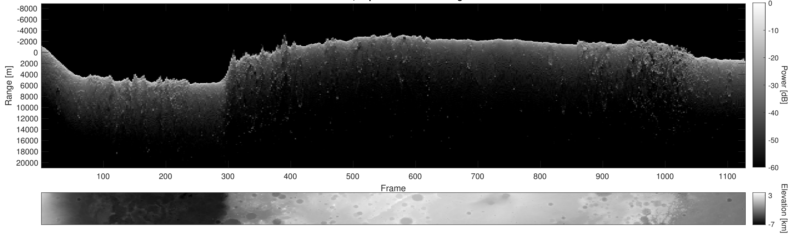
Orbit 22917, Depth-Corrected Cluttergram
