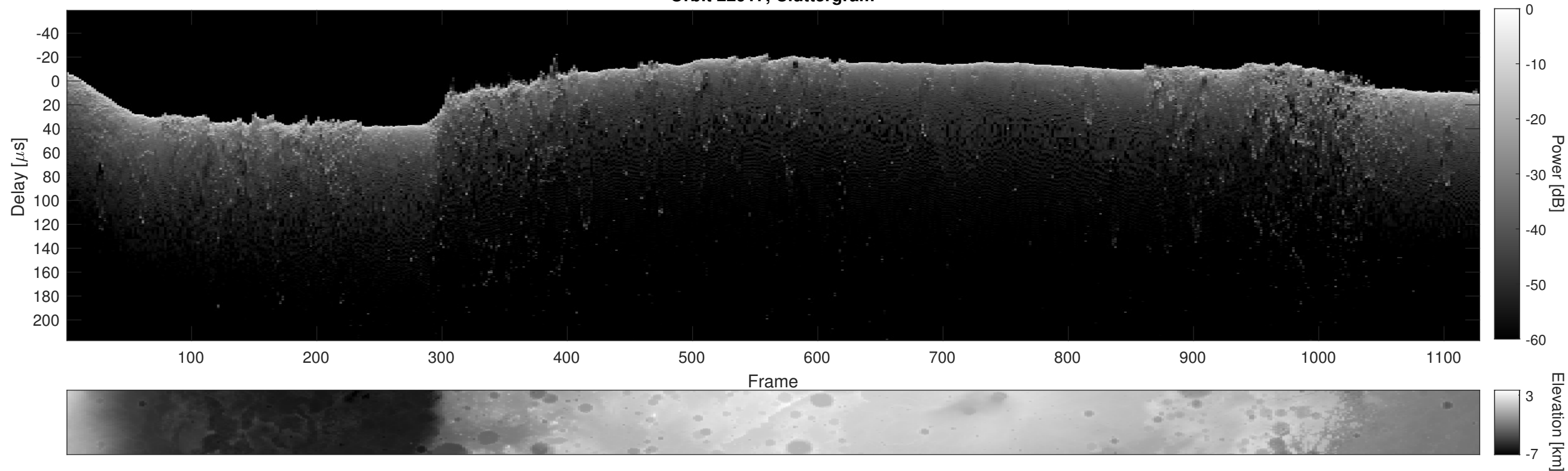
Orbit 22917, Cluttergram
