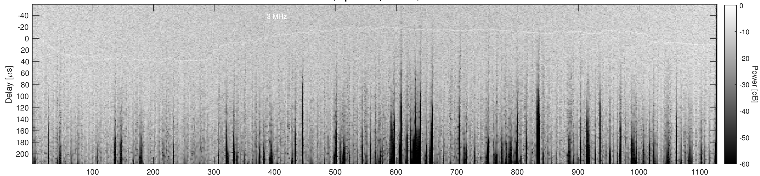
Orbit 22917, Cluttergram
