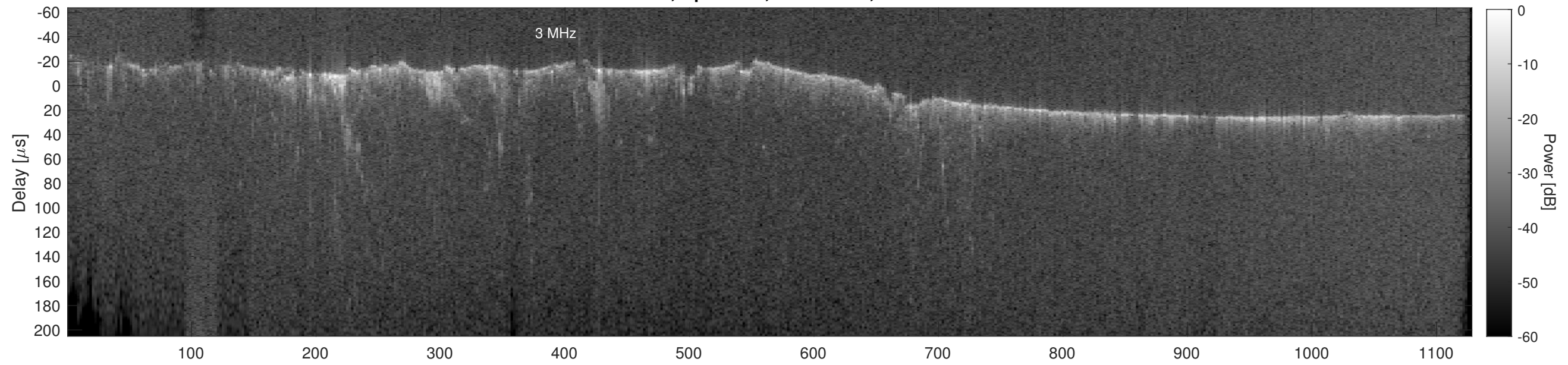
Orbit 22920, Cluttergram
