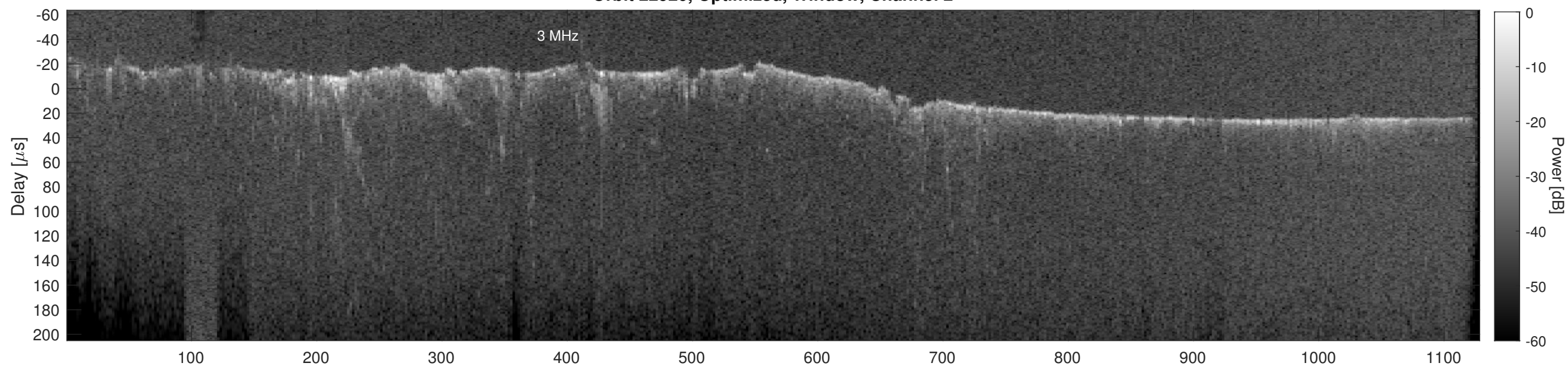
Orbit 22920, Cluttergram
