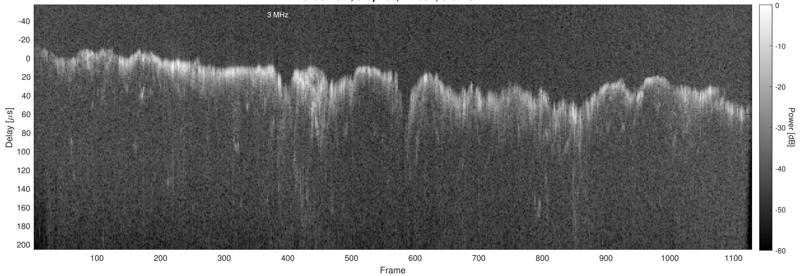
Orbit 22921, Chapman, Window, Channel 2
