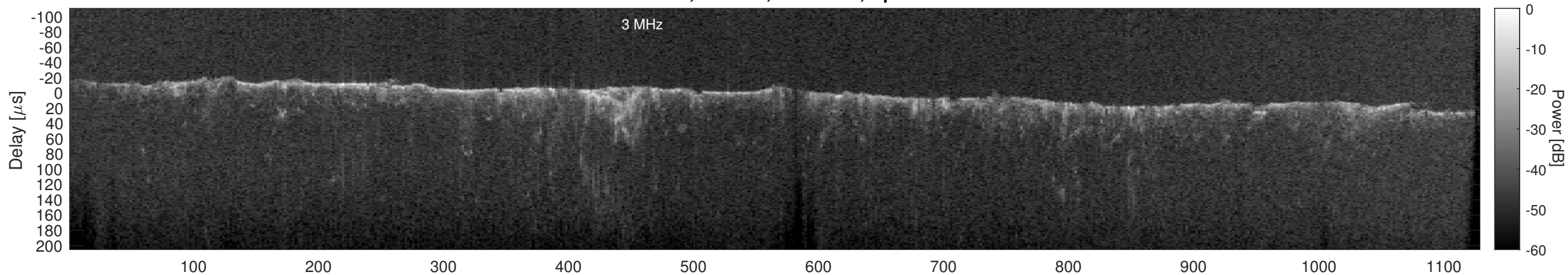
Orbit 22921, Cluttergram
