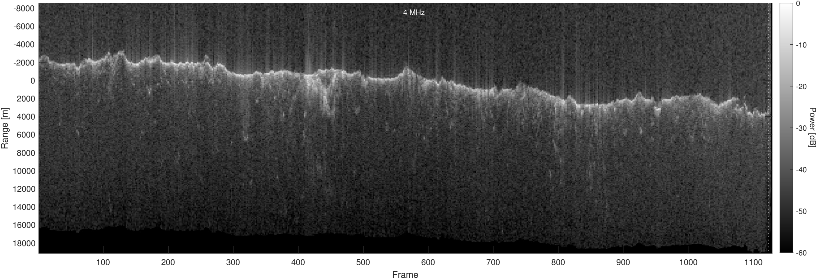
Orbit 22921, Optimized, No Window, Depth-Corrected, Channel 2
