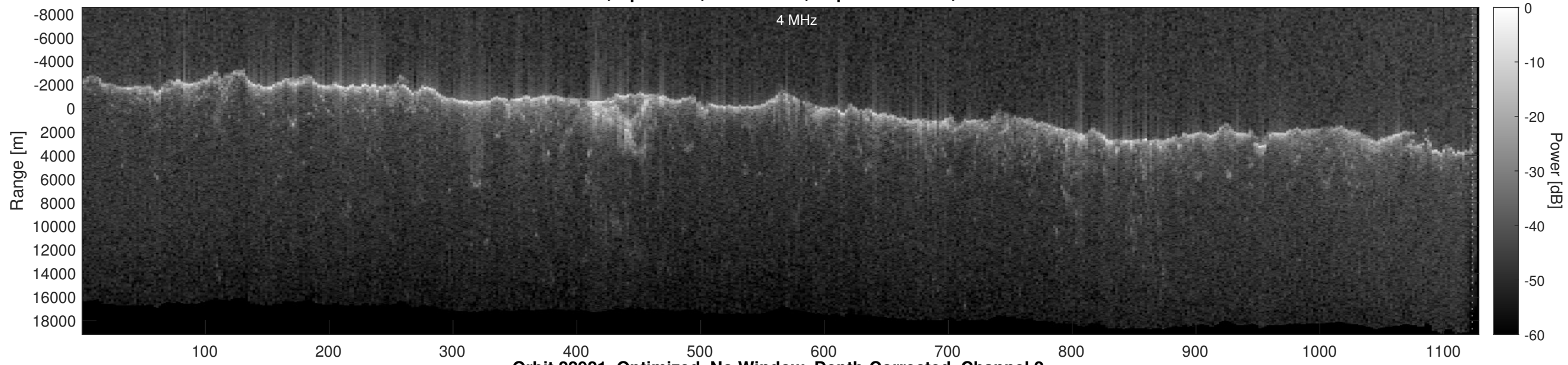
Orbit 22921, Optimized, No Window, Depth-Corrected, Channel 2
