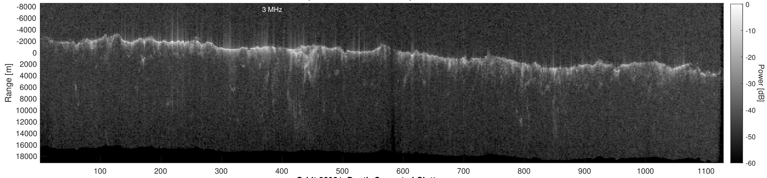
Orbit 22921, Depth-Corrected Cluttergram
