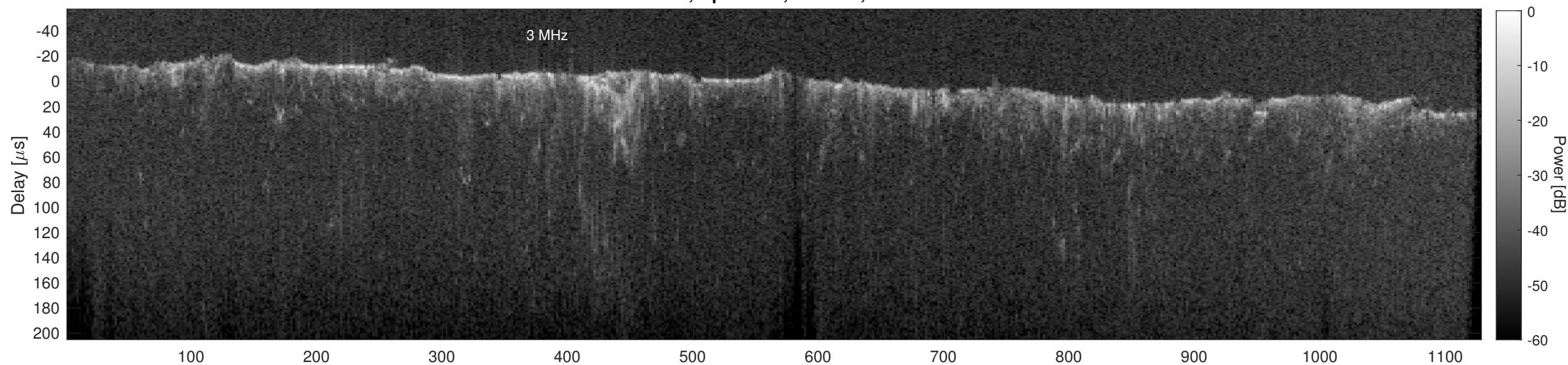
Orbit 22921, Cluttergram
