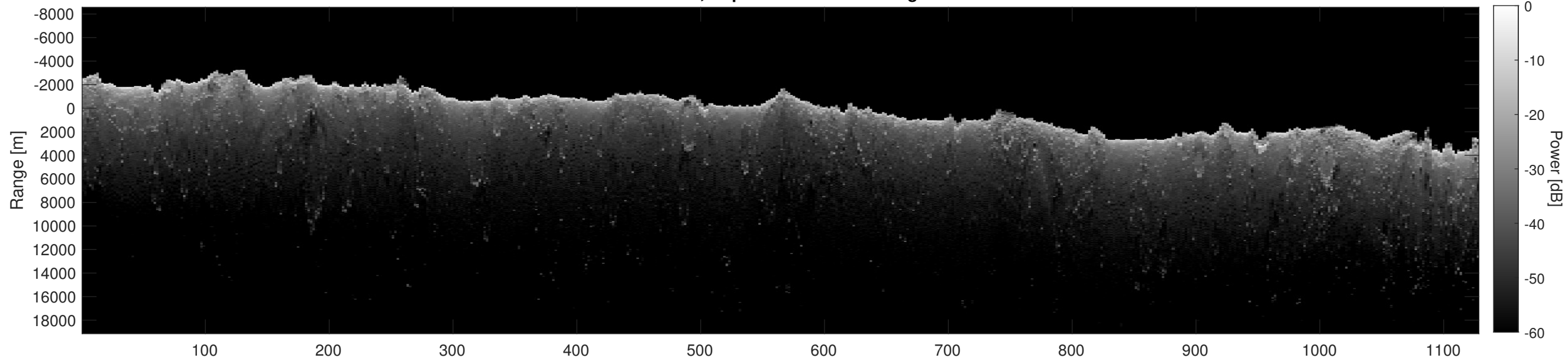
Orbit 22921, Depth-Corrected Cluttergram
