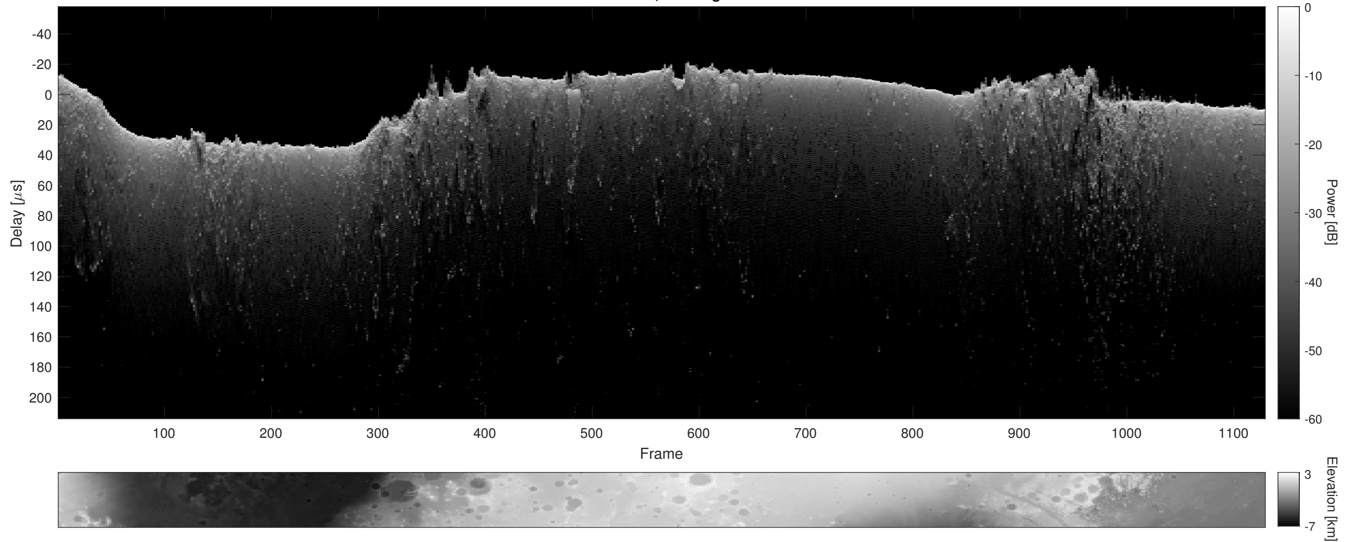
Orbit 22924, Cluttergram
