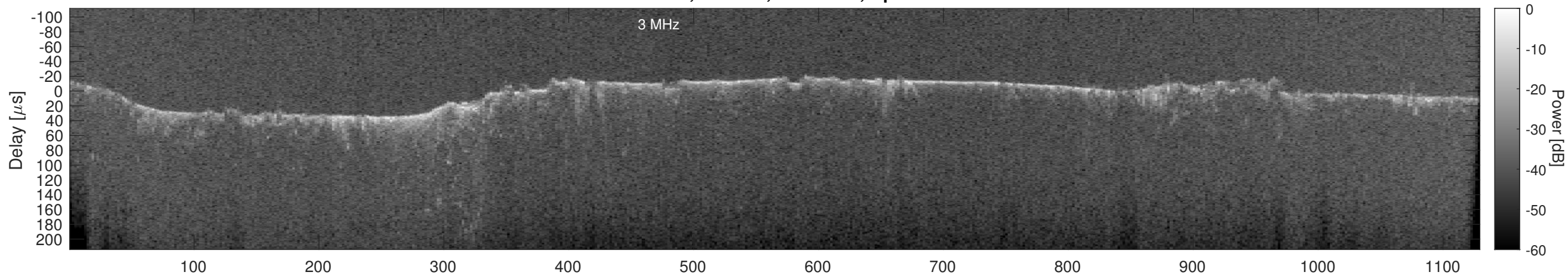
Orbit 22924, Cluttergram
