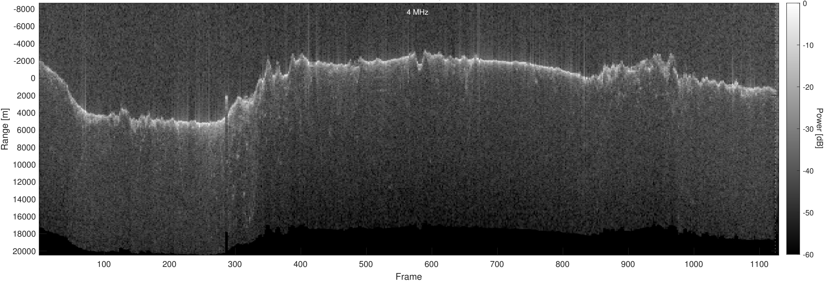
Orbit 22924, Optimized, No Window, Depth-Corrected, Channel 2
