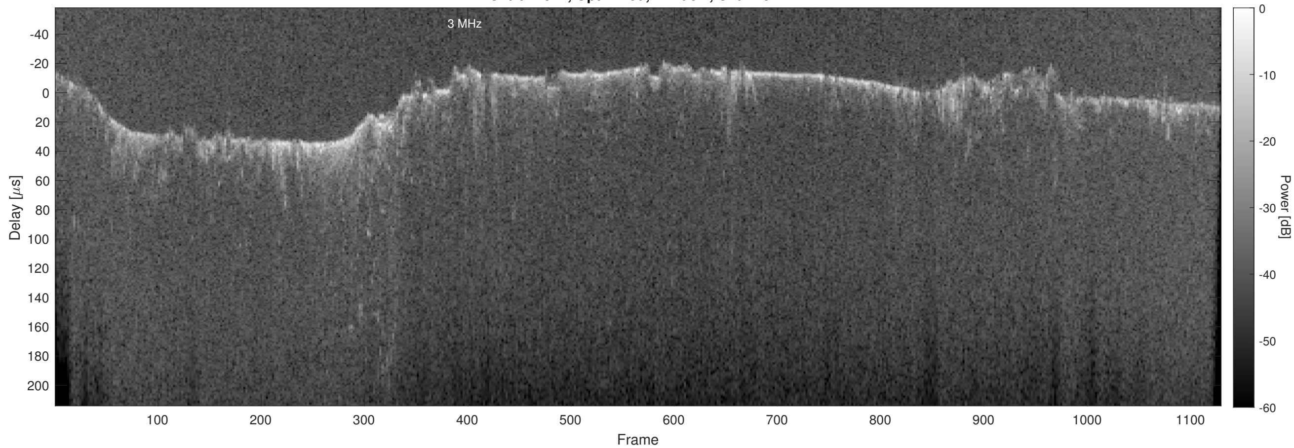
Orbit 22924, Optimized, Window, Channel 2
