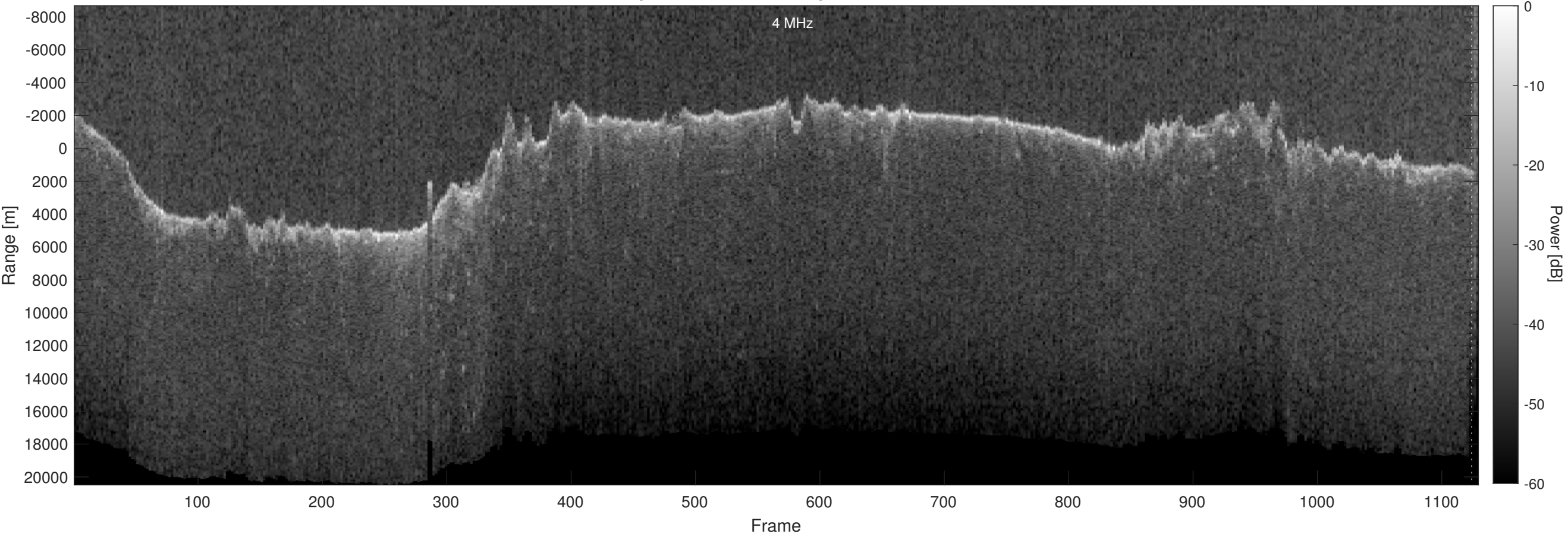
Orbit 22924, Optimized, Window, Depth-Corrected, Channel 2
