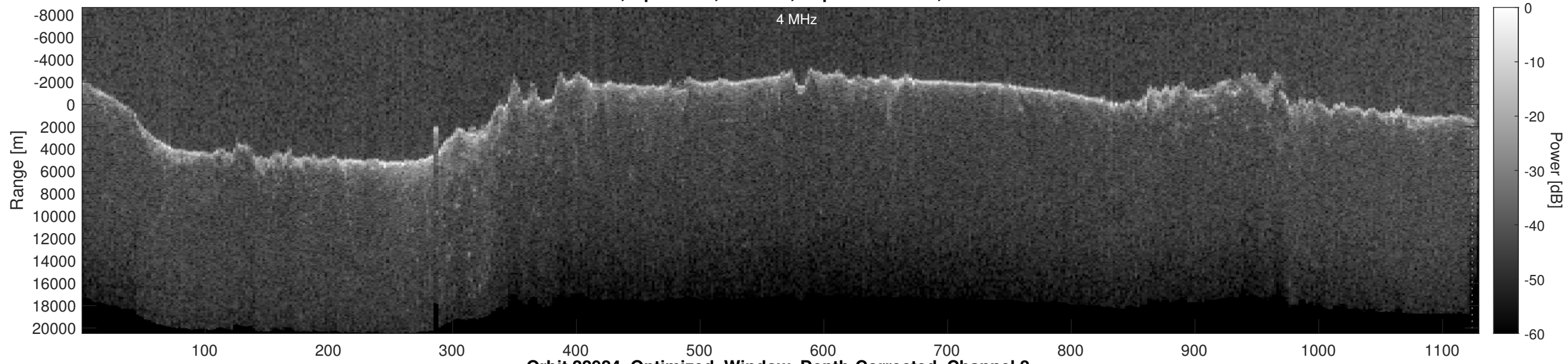
Orbit 22924, Optimized, Window, Depth-Corrected, Channel 2
