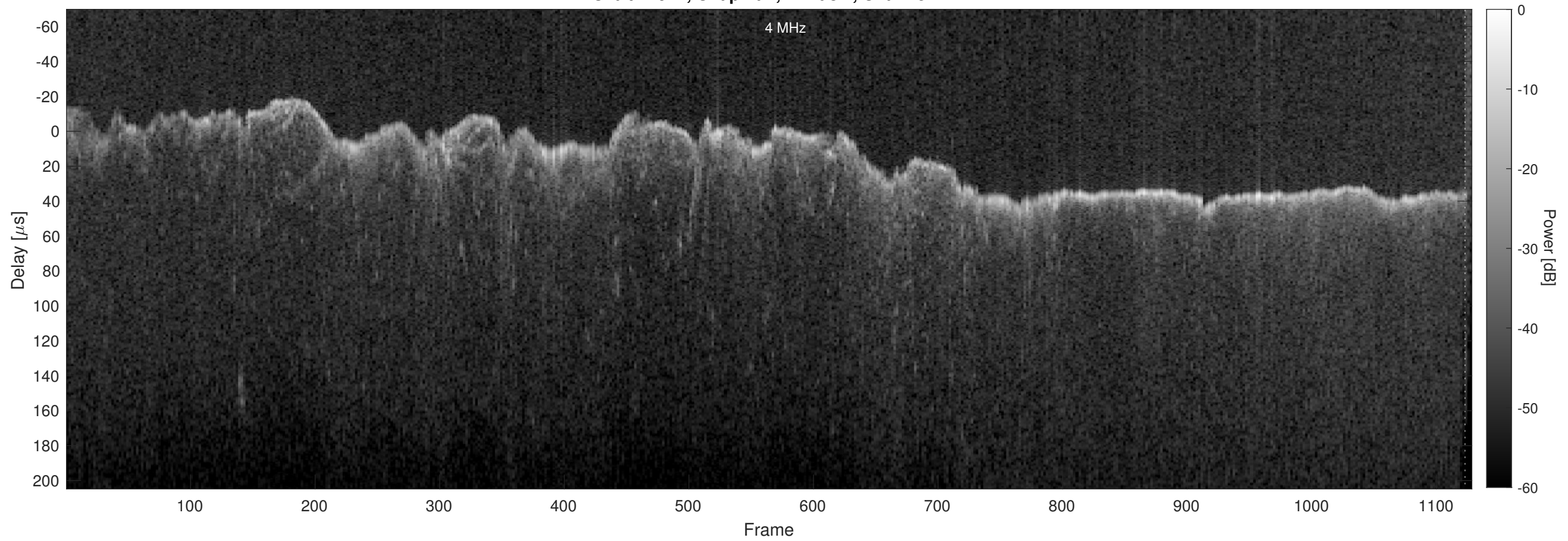
Orbit 22927, Chapman, Window, Channel 2
