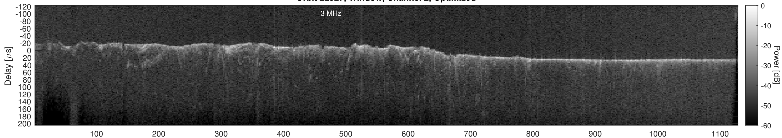
Orbit 22927, Cluttergram
