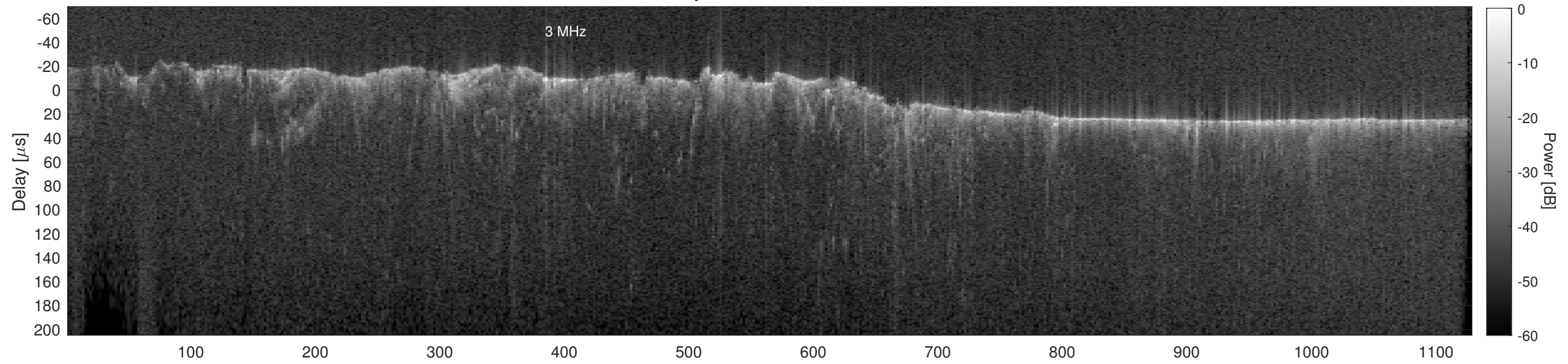
Orbit 22927, Cluttergram
