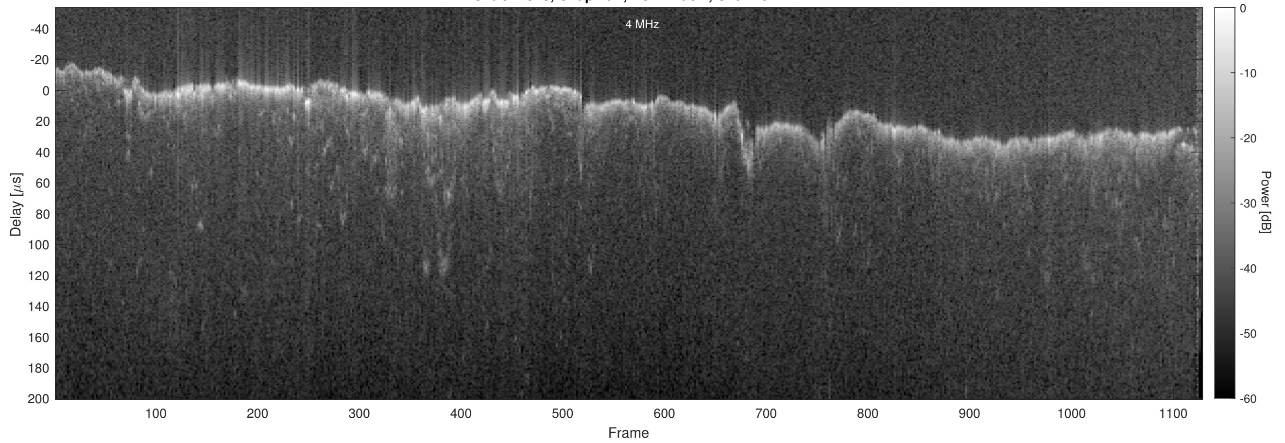
Orbit 22928, Chapman, No Window, Channel 2
