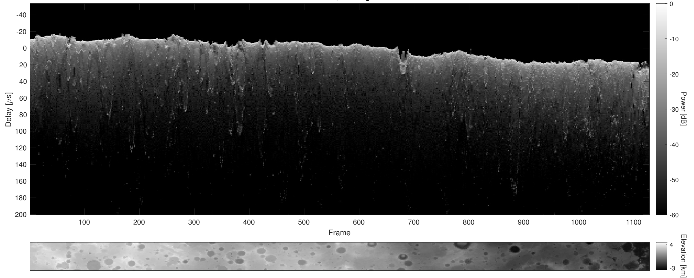
Orbit 22928, Cluttergram
