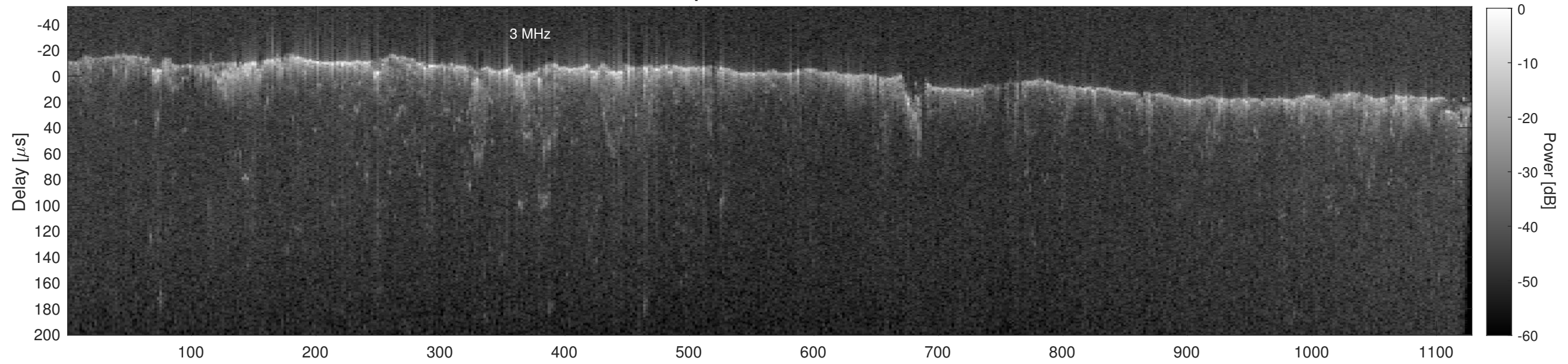
Orbit 22928, Cluttergram
