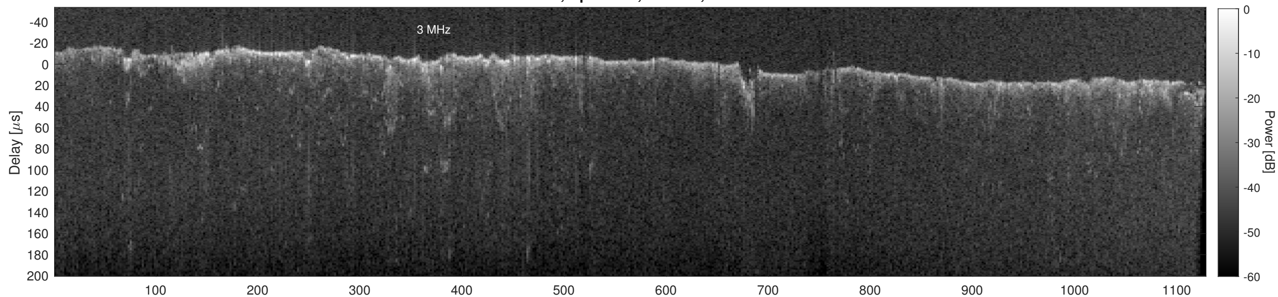
Orbit 22928, Cluttergram
